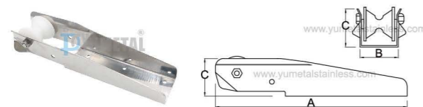
S.M0425 Anchor Bow Roller Stainless Steel AISI316
