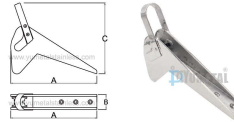
S.M0401 Anchor Bow Roller Stainless Steel AISI316
