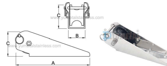
S.M0428 Anchor Bow Roller Stainless Steel AISI316
