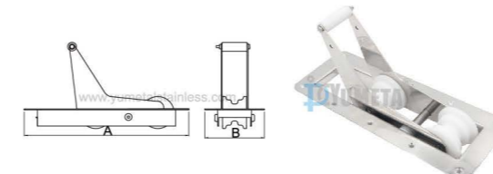
S.M0430 Anchor Bow Roller Stainless Steel AISI316
