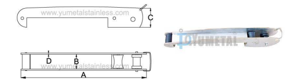
S.M0418 Anchor Bow Roller Stainless Steel AISI316
