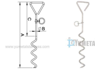
S.AN13 Ground Anchor
