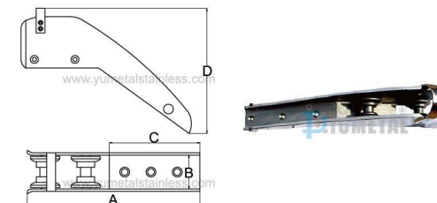
S.M0417 Anchor Bow Roller Stainless Steel AISI316
