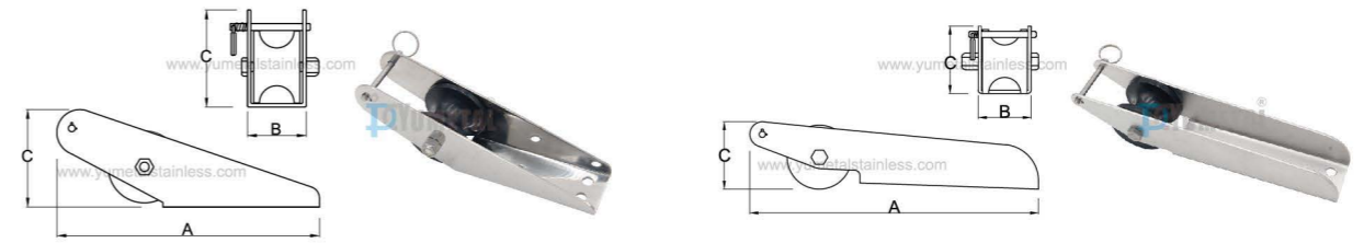
S.M0427 Anchor Bow Roller Stainless Steel AISI316
