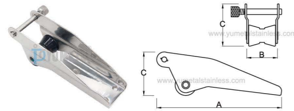
S.M0419 Anchor Bow Roller Stainless Steel AISI316
