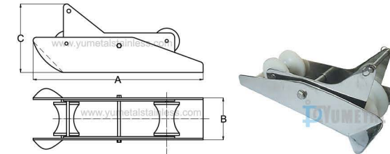
S.M0403 Anchor Bow Roller Stainless Steel AISI316
