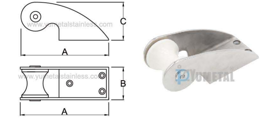
S.M0402 Anchor Bow Roller Stainless Steel AISI316
