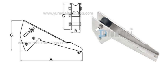
S.M0429 Anchor Bow Roller Stainless Steel AISI316
