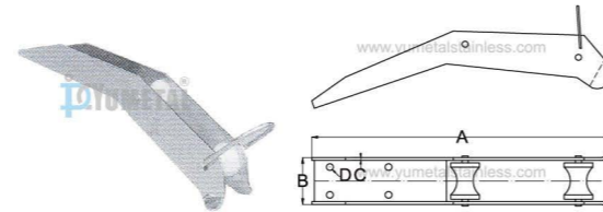
S.M0424 Anchor Bow Roller Stainless Steel AISI316
