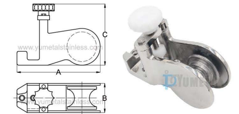
S.M0404 Anchor Bow Roller Stainless Steel AISI316
