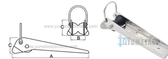
S.M0415 Anchor Bow Roller Stainless Steel AISI316
