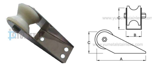
S.M0408 Anchor Bow Roller Stainless Steel AISI316
